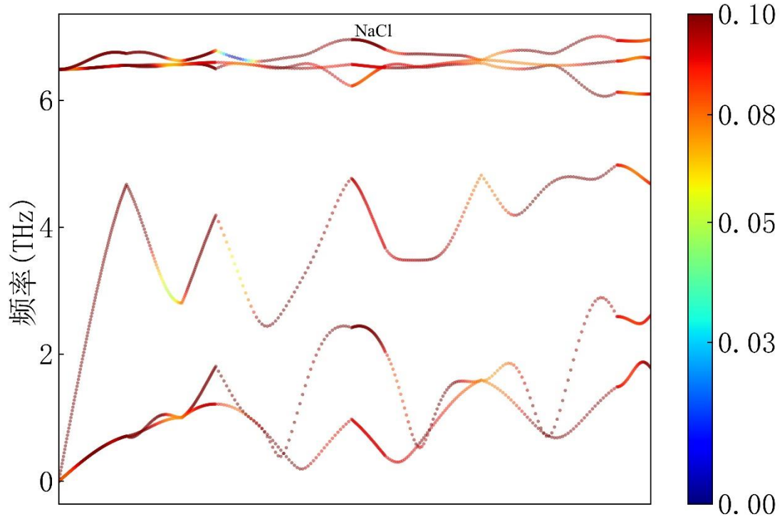
图 S8 NaCl 晶体的声子谱，图中点的颜色值为对应声子模式的非简谐性描述符 \sigma_{q,j}^A Fig. S8. Phonon spectra of NaCl, with color value of point denoting anharmonic descriptor \sigma_{q,j}^A of corresponding phonon mode.
