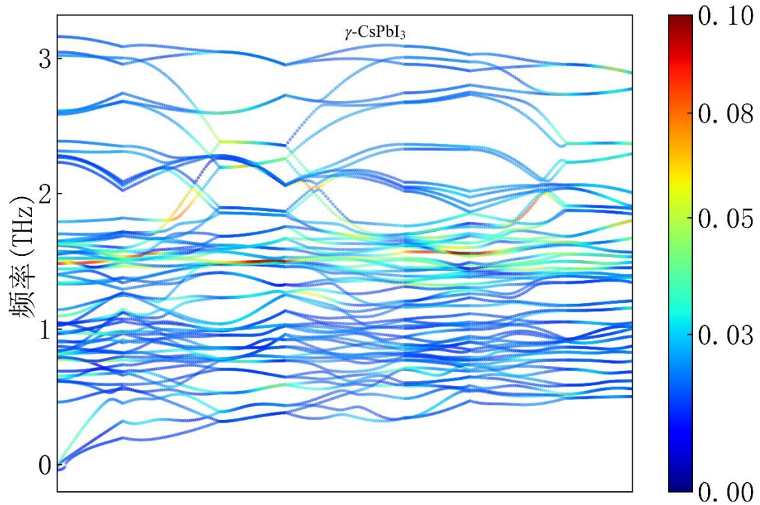
图 S9 \gamma -CsPbI 3 晶体的声子谱，图中点的颜色值为对应声子模式的非简谐性描述符 \sigma_{q,j}^A Fig. S9. Phonon spectra of \gamma -CsPbI 3 , with color value of point referring to anharmonic descriptor \sigma_{q,j}^A of corresponding phonon mode.
